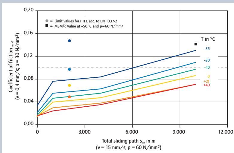
Figure B: MSM®-strips in long term sliding test (without dimples)
