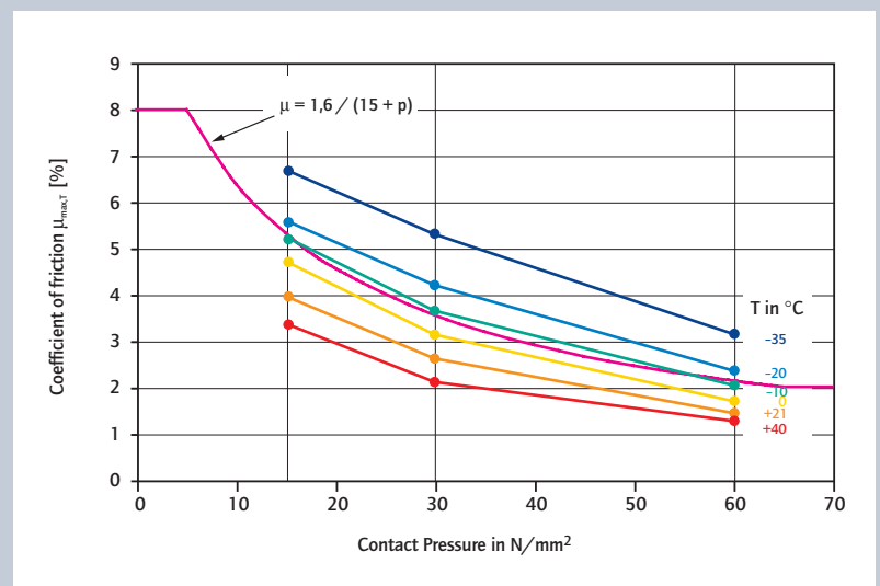
Figure E: Coefficients of friction of MSM®-sheets with dimples as a function of contact pressure
