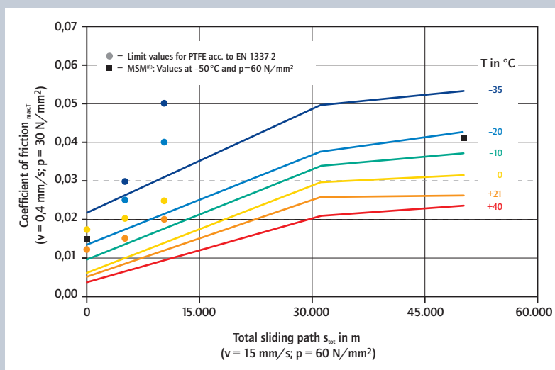
Figure A: MSM®-sheets in long term sliding test (with dimples)
