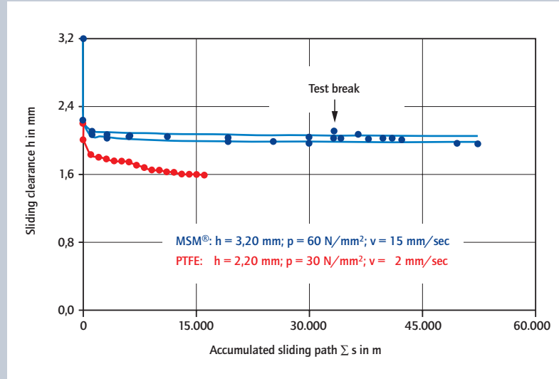
Figure C: Wear in the same long term test as in Figure A
